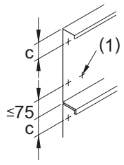
Clearance to side of sheet
