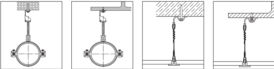
Threaded rod attachments to concrete and steel
