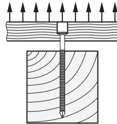
Head pull-through f_{head,k}
