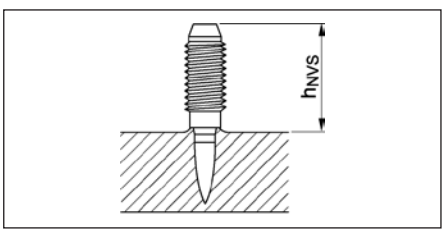
X-ST-GR M8/5 P8, h_{NVS} = 12.0 - 15.0 \text{ mm} X-ST-GR M8/10 P8, h_{NVS} = 17.0 - 20.0 \text{ mm}
